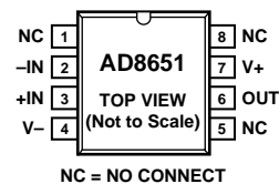
Figure 3. 8-Lead SOIC (R-8)
